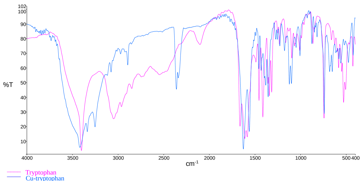
Figure 4: Comparative FT IR spectra of of tryptophan and Cu- tryptophan complex
